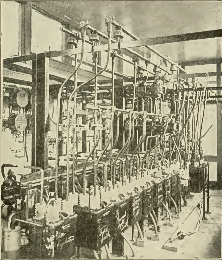
Fig. 158. Switchboard of the St. Clair Tunnel Power Plant, Rear View
